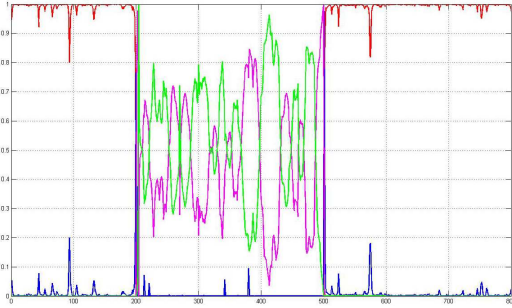
Fig. 4. Confidence values of activity states, t \in [1 \dots T] : “inactive” (red), “low movement” (blue), “medium movement” (magenta), “intense movement” (green).
