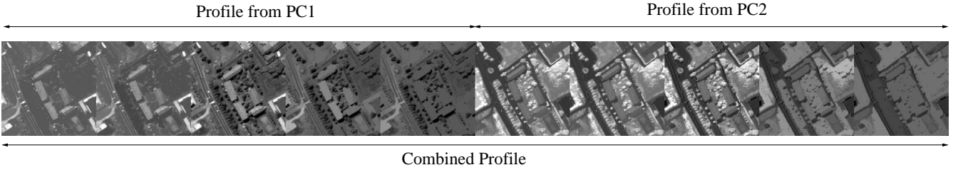
Fig. 2. Extended morphological profile of two images. Each of the original profiles has 2 opening and 2 closings. A circular structuring element with radius increment 4 was used ( r = 4, 8 ). The image processed is part of Fig. 4.(a).
