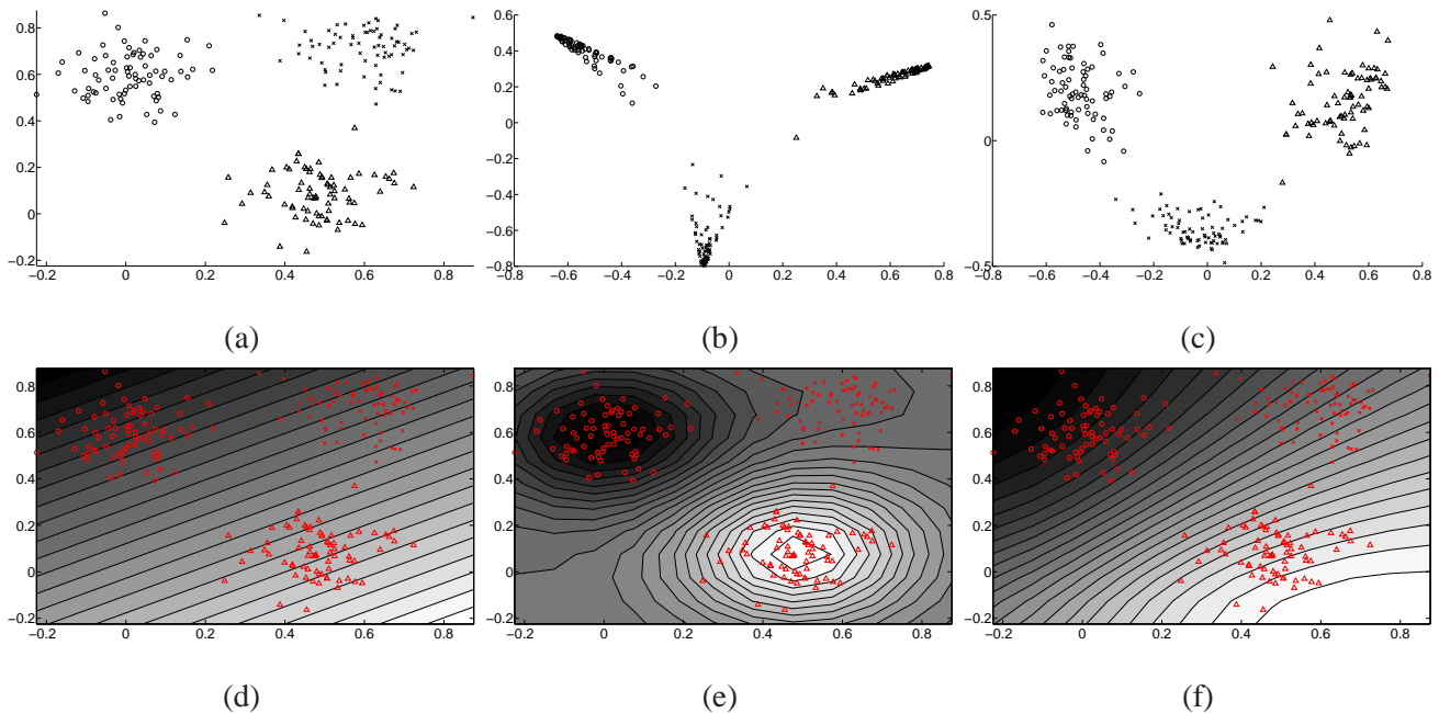
Fig. 3. PCA versus KPCA: (a) Three Gaussian clusters, and their projection onto the first two kernel principal components with (b) a Gaussian kernel and (c) a polynomial kernel. (d), (e) and (f) represent, respectively, the contour plot of the projection onto the first component for the PCA, the KPCA with Gaussian kernel and the KPCA with a polynomial kernel. Note how with the Gaussian kernel the first component ‘picks out’ the individual clusters [20]. The intensity of the contour plot is proportional to the value of the projection, i.e. , light gray indicates that \Phi_{kpc}^1(\mathbf{x}) has a high value.
