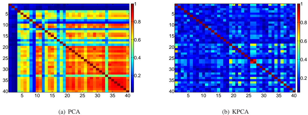
Fig. 5. Mutual Information matrices for the Washington DC data set.
