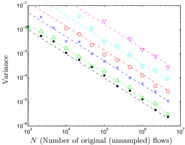
Figure 3: Variance of the MLE estimator against number of original flows considered ( \alpha = 1.5 ) for different values of N and j_{\min} : ( \bullet , black) p = \frac{1}{10} , j_{\min} = 0 - ( \Delta , green) p = \frac{1}{10} , j_{\min} = 1 - ( \times , blue) p = \frac{1}{100} , j_{\min} = 0 - ( \circ , red) p = \frac{1}{100} , j_{\min} = 1 - ( \diamond , cyan) p = \frac{1}{1000} , j_{\min} = 0 - ( \nabla , magenta) p = \frac{1}{1000} , j_{\min} = 1 . The dash-dotted plots represents the theoretical lower bound of the variance (Cramér-Rao bound).
