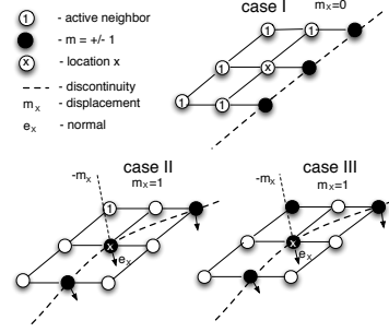
Fig. 1. The figure shows how the neighborhood is activated based on \mathbf{A} = (\mathbf{M}, \mathbf{E})
