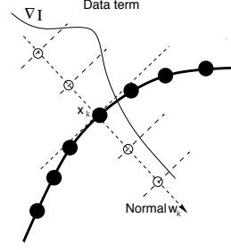
Fig. 2. The figure shows the calculation of U_c using gradient information
