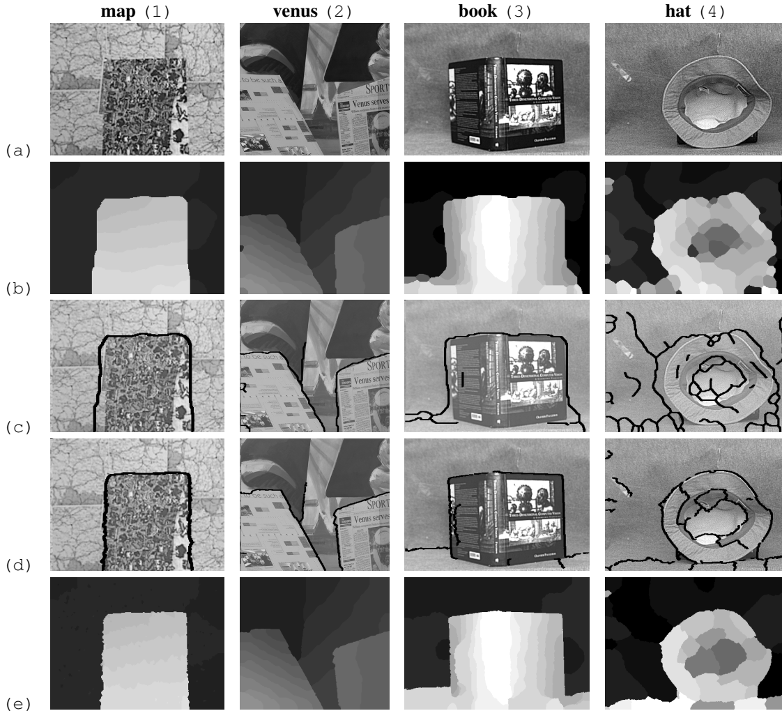
Fig. 3. (a) Original Images; (b) Disparity maps using Variational Mean-field only; (c) Disparity discontinuities corresponding to (b); (d) Corrected disparity discontinuities using our approach; (e) Corresponding disparity maps.
